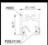
P20E TOP TRACK ONE-PIECE CONSTRUCTION
