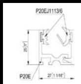
P20E TOP OR BOTTOM TRACK TWO-PIECE CONSTRUCTION
