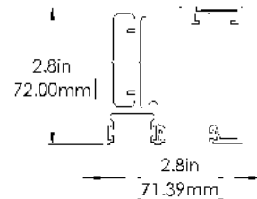
Top Track
